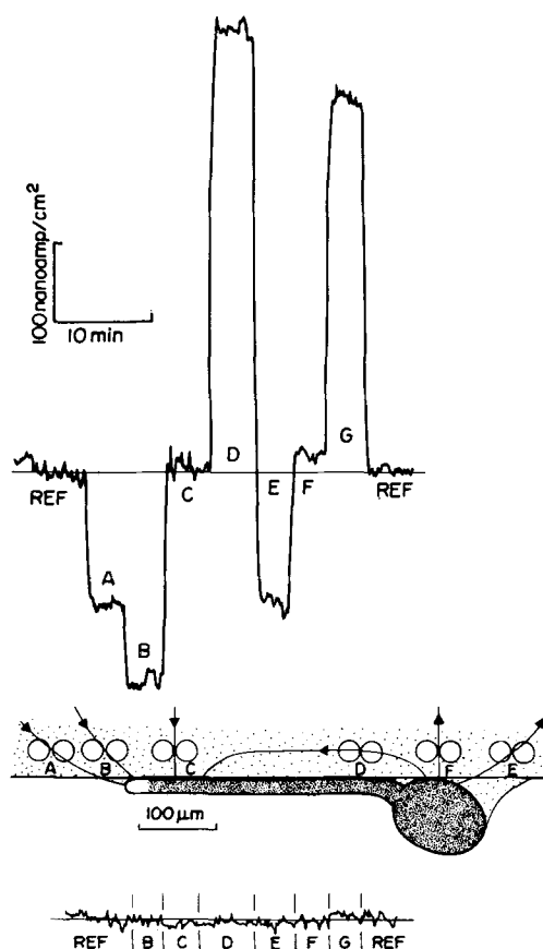
FIGURE 2 Representative recording of the axial field near a young, growing pollen tube and grain. Top: Actual recording; downward movement of the trace indicates rightward movement of the current in the diagram. Middle: Scale diagram of the pollen tube and grain in side view. Drawn near the end of the recording when the tube was 350 \mu\text{m} long; when the recording began, it was 150 \mu\text{m} long. It grew at 6–7 \mu\text{m}/\text{min} during the recording. The vibrating probe is represented by two circles. Pairs A–C are drawn to show their position with reference to the tip; D–F, the grain. Lines with arrows symbolize the inferred current. Bottom: Control recording from a similar tube after fixation in glutaraldehyde.
